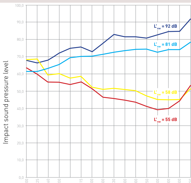
Figure 6. Through the frequency spectrum, the figure above shows how a floating screed with Isolmant MonoPlus or Isolmant UnderPlus Black.E (yellow line) or Isolmant BiPlus or Isolmant UnderSpecial (red line) can improve impact sound insulation of a bare hollow clay slab (blu line) or a traditional bounded screed (cyan line).
