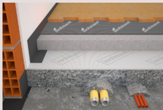
Base slab Levelling screed Isolmant Underscreed Screed Isolmant IsolTile Wooden Flooring
